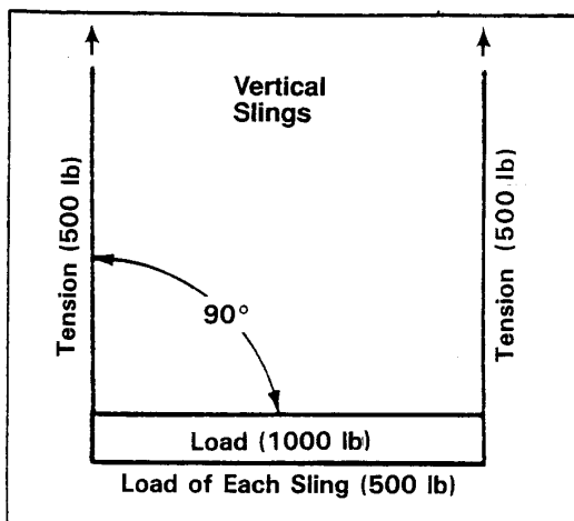
Figure 9-1. Sling Stresses at Various Sling Angles (Sling Angles Less than 30E Not Recommended).
