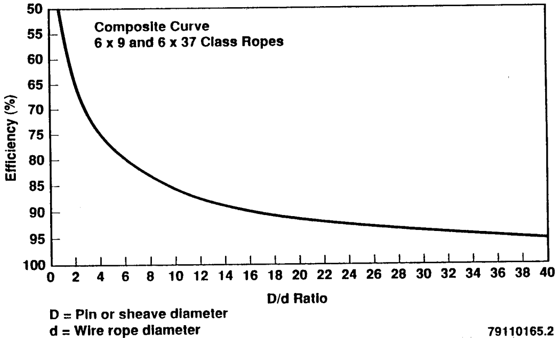
Figure 9-5. Wire Rope Efficiencies for Various D/d Ratios.
