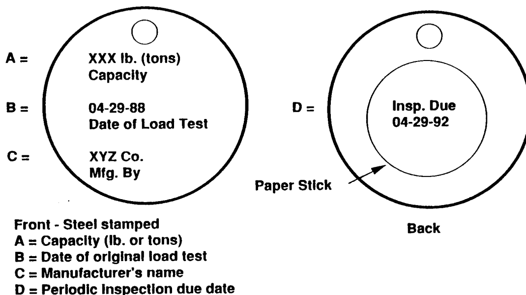
Figure 9-6. Rigging Tackle and Equipment Identification Tag Example.
